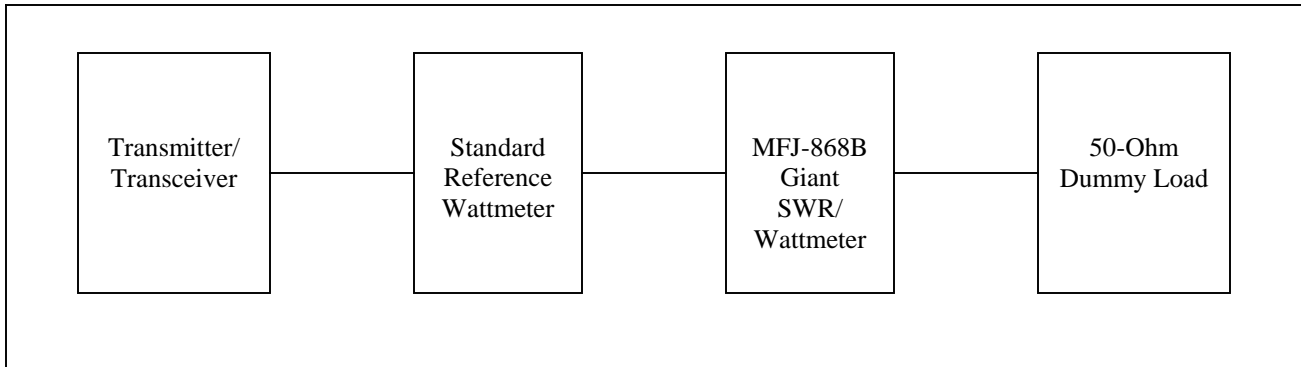
Figure 3: Calibration Setup
